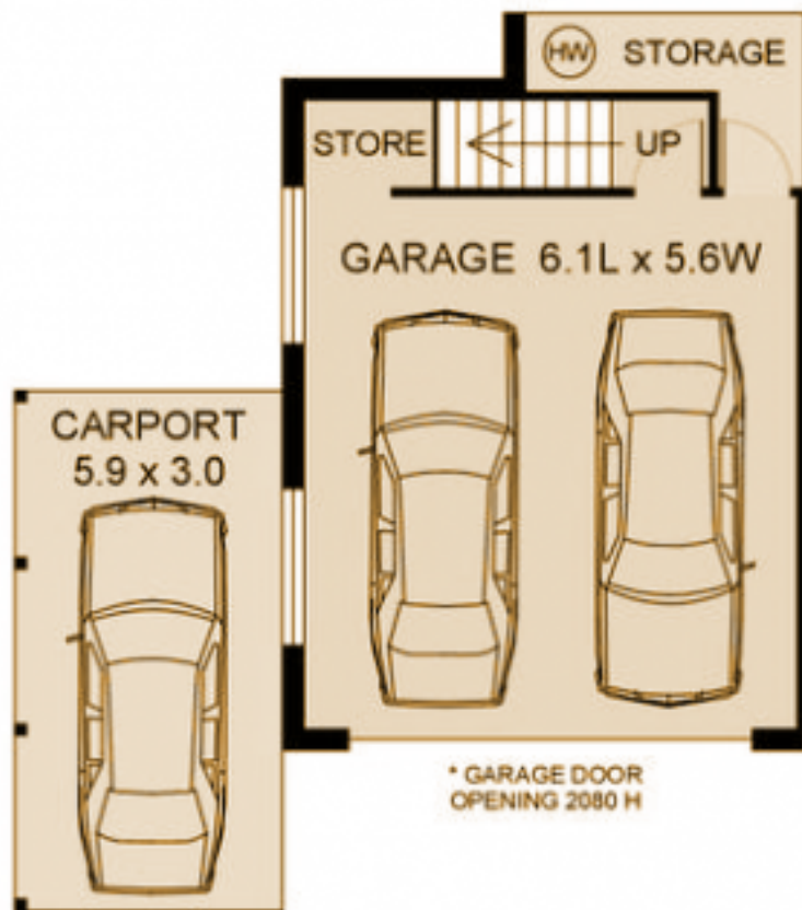
LOWER FLOOR PLAN (44 sq m Approx)
